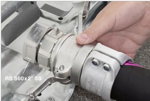
Reduzierstück RS S60x2" SS mit Camlock Kupplung AVKI 50 SS Female reducer RS S60x2" SS with Cam Locking Coupling AVKI 50 SS
